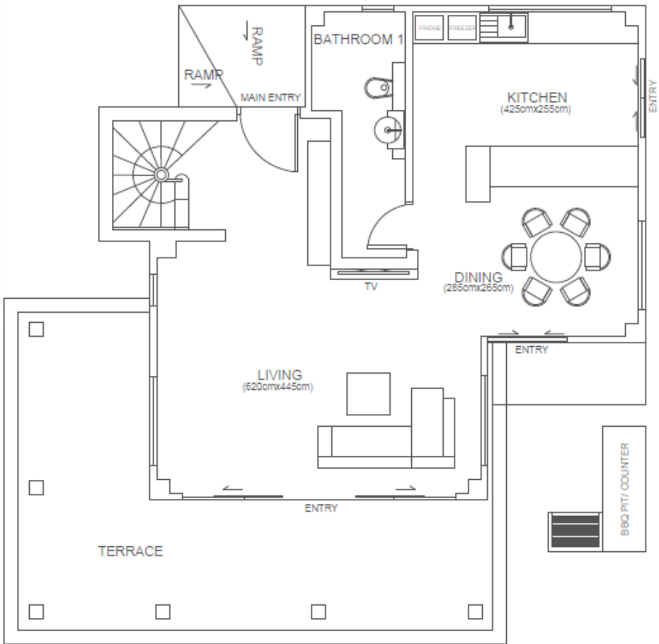
1 ST STOREY LAYOUT PLAN
